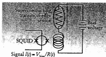
FIGURE 4. SCHEMATIC bias circuits for two kinds of resistive thermometer. A semiconductor thermistor (left) shows a decrease in resistance with increasing temperature, whereas a superconducting transition-edge sensor (right) increases in resistance with increasing temperature within its superconducting transition. The choice of constant current bias for the former and constant voltage bias for the latter results in both devices exhibiting negative electrothermal feedback—that is, the Joule power ( I^2 R = V^2/R ) decreases as the temperature is raised.
